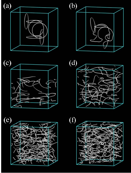
FIG. 1. (Color online) Development of a vortex tangle by the full Biot-Savart calculation in a periodic box with a size of 0.1 cm. Here, the temperature is T=1.9 K and the counterflow velocity v_{ns}=0.572 cm/s is along the vertical axis. (a) t=0 s, (b) t=0.05 s, (c) t=0.5 s, (d) t=1.0 s, (e) t=3.0 s, and (f) t=4.0 s.
