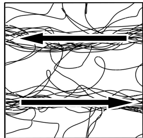
FIG. 10. Vorticity direction of bundles in the layer vortices shown in Figs. 6(a) and 6(c).
