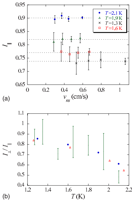
FIG. 5. (Color online) (a) Anisotropy parameter I_{\parallel} as a function of v_{ns} . The error bars represent the standard deviation. (b) Anisotropy ratio I_{\perp}/I_{\parallel} as a function of temperature obtained by us (dots), Schwarz (Ref. 13) (triangles), and experimentally (Ref. 23) (vertical bars).
