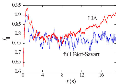
FIG. 8. (Color online) Comparison of the time evolution of the anisotropy parameter I_{||}(t) for the simulation of Fig. 6.
