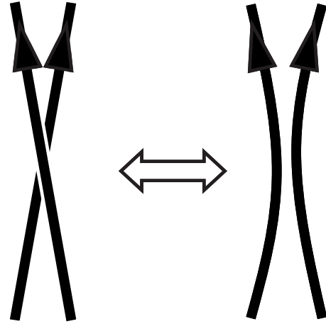
FIG. 9. Reconnection of almost parallel vortices.
