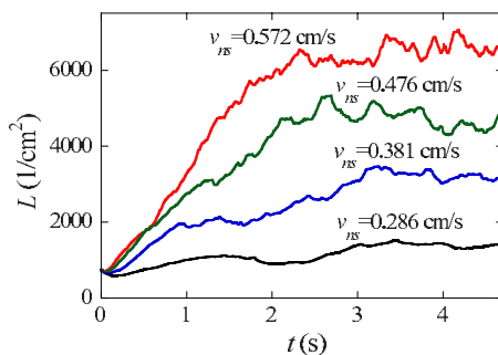
FIG. 2. (Color online) Vortex line density as a function of time for four different counterflow velocities.
