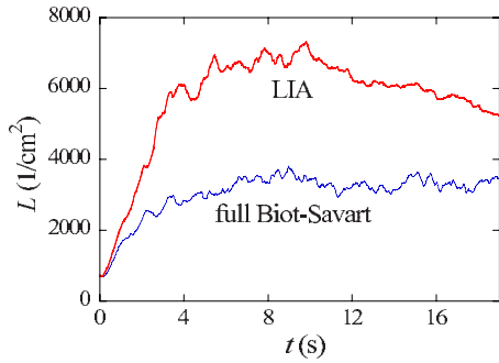
FIG. 7. (Color online) Comparison of the time evolution of the vortex line density L(t) for the simulation of Fig. 6.
