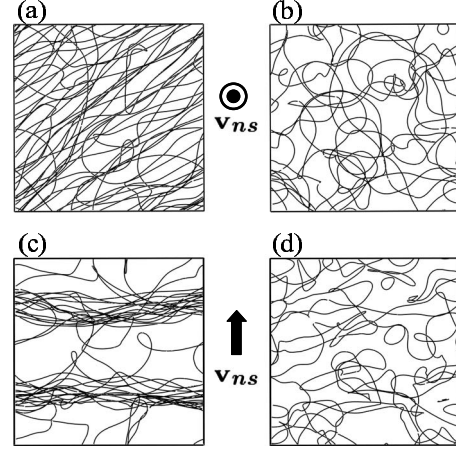
FIG. 6. (a) Side and (c) top views of the LIA calculation. (b) Side and (d) top views of the full Biot-Savart calculation. All figures are at t=18.6 s. The system is a (0.2 \text{ cm})^3 cube. Applied normal-fluid velocity is v_{ns}=0.55 \text{ cm/s} .
